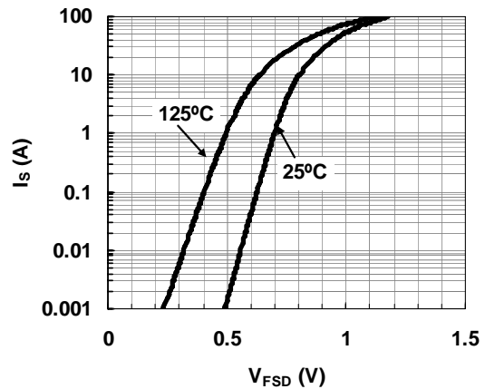
Figure 6. Body Diode Forward Voltage versus Source Current
