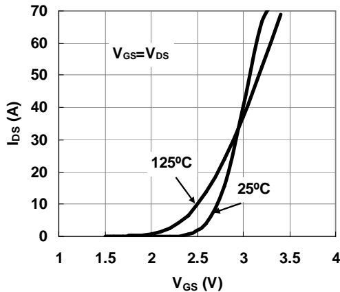
Figure 5. Transfer Characteristics
