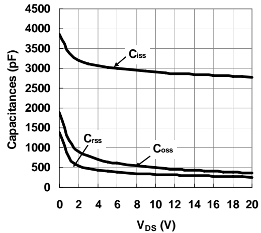
Figure 10. Capacitance Characteristics
