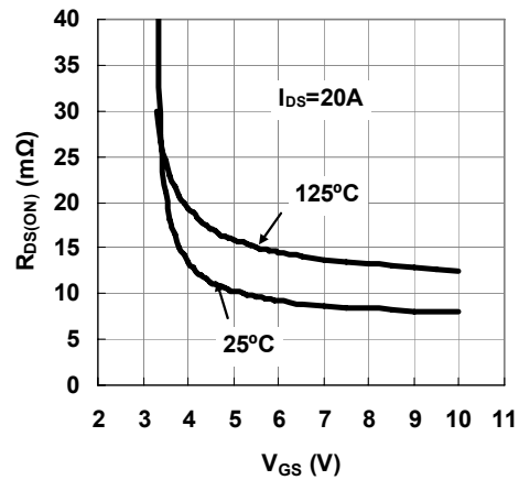
Figure 4. On-Resistance versus Gate to Source Voltage
