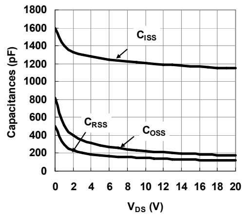
Figure 10. Capacitance Characteristics
