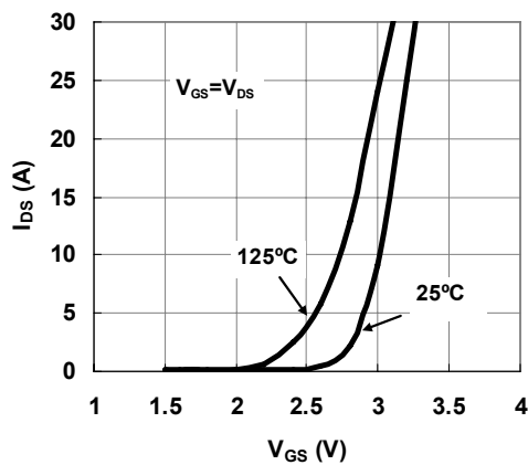
Figure 5. Transfer Characteristics
